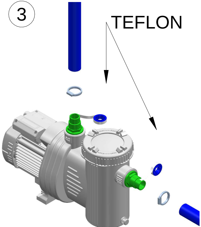
Hoses connection
