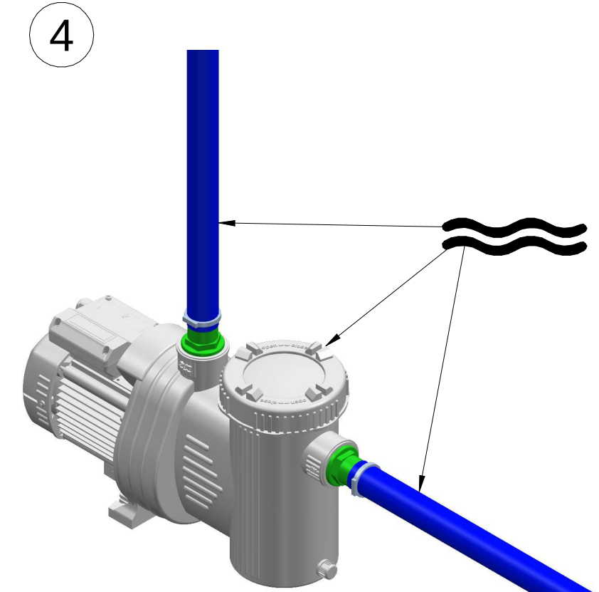
Filling water
